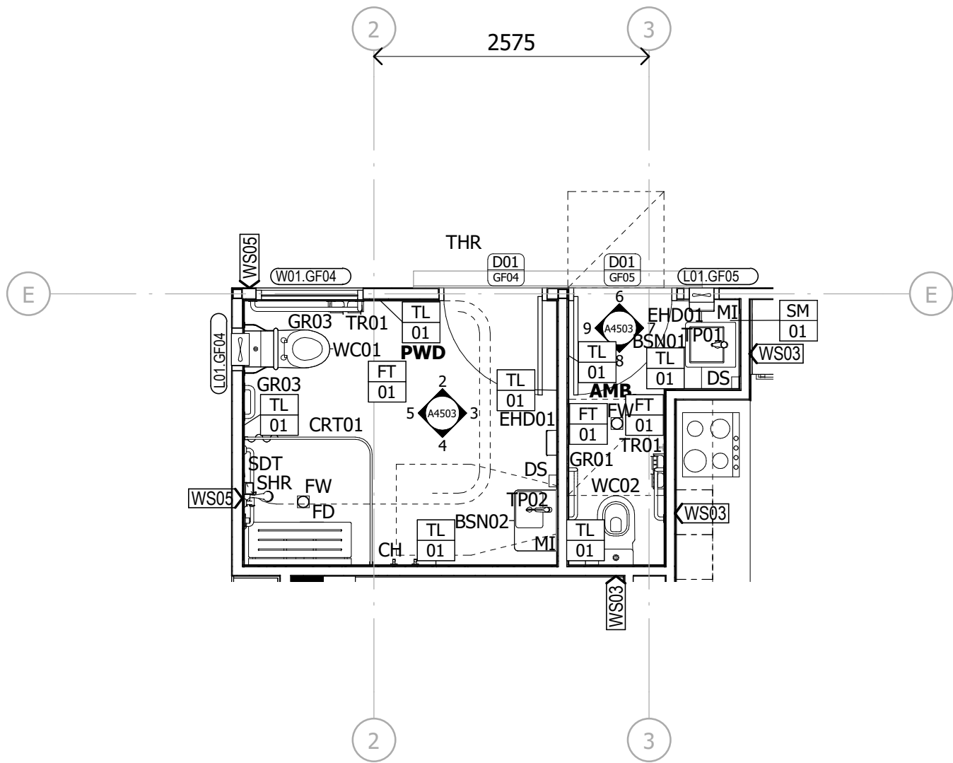
1 GA PLAN - AMENITIES A2001 1 : 50
